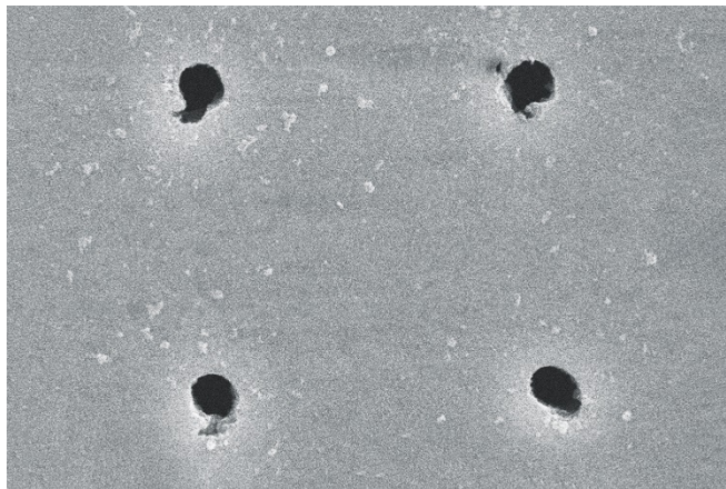
Image 3: Holes with exit diameter of one micrometer in 10 micrometer thick stainless steel foil with 10 micrometer spacing. © Fraunhofer ILT, Aachen, Germany.
