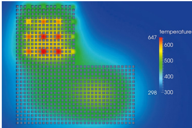
Image 2: Simulation of the thermal propagation during USP multibeam processing. © Fraunhofer ILT, Aachen, Germany.
